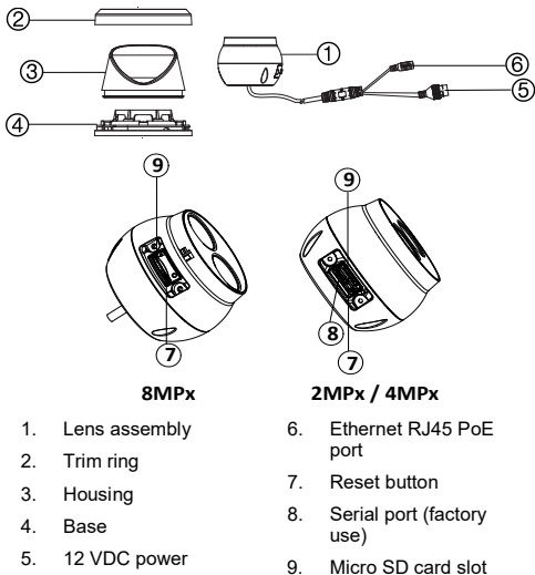
Figure 3: IP fixed lens turret camera
