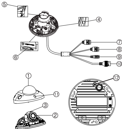
Figure 7: IP fixed lens wedge camera
